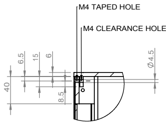
DETAIL M SCALE 1 : 5
