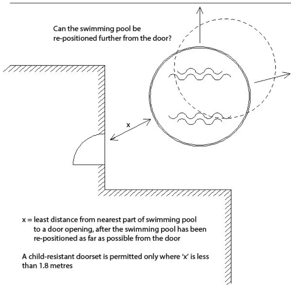
Figure 3.1.3b Above-ground swimming pool (including spa pools)
