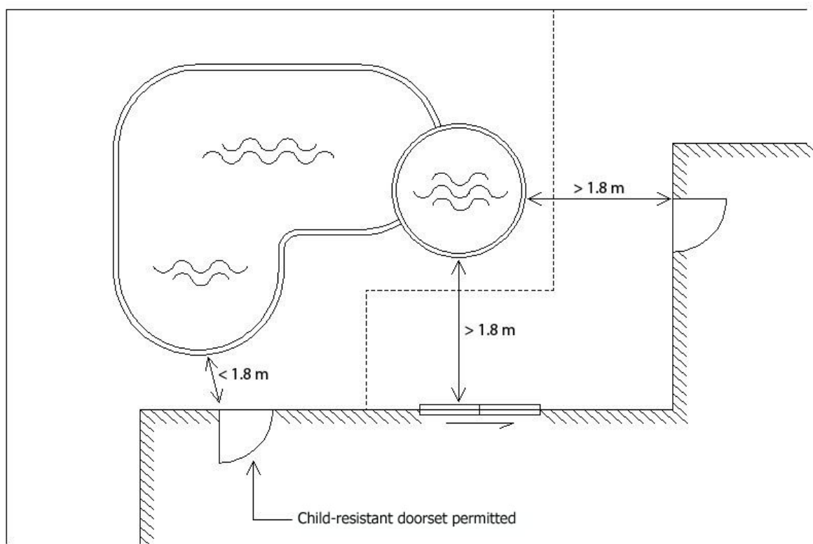
Figure 3.1.3a – In-ground swimming pools (including spa pools).
