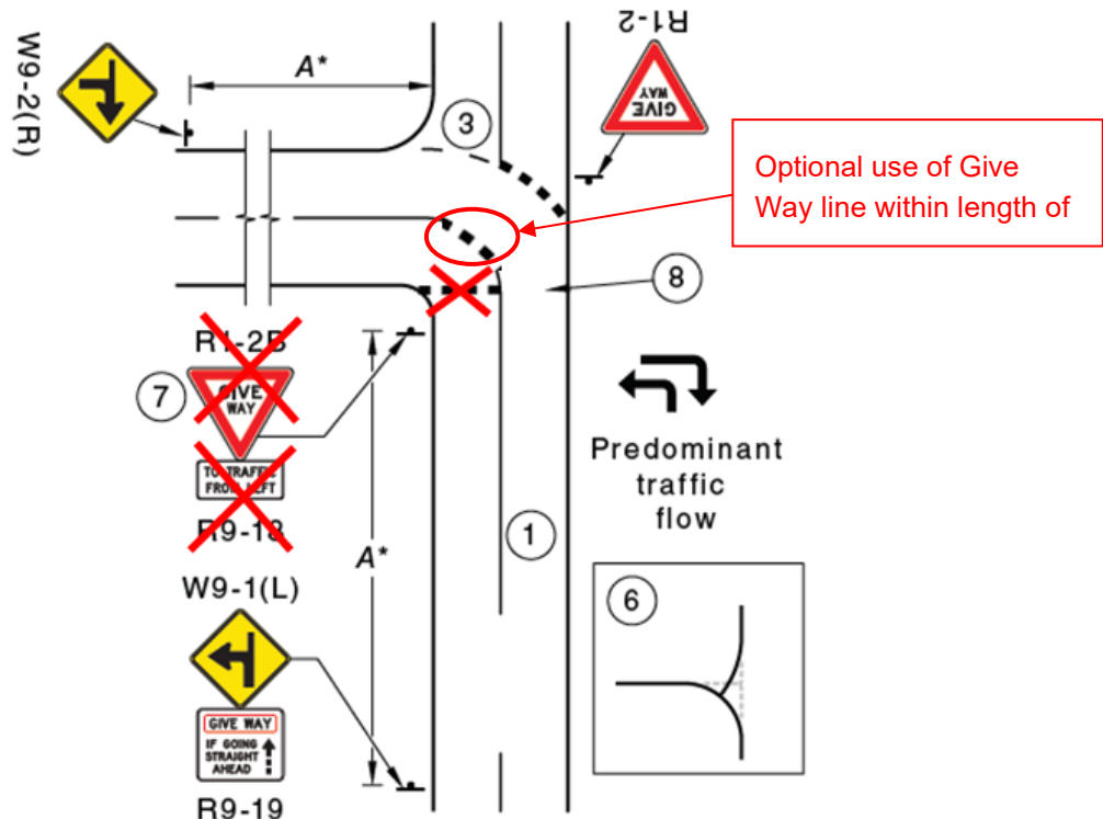
(c) T-intersection: interim treatment where raised island is not possible
