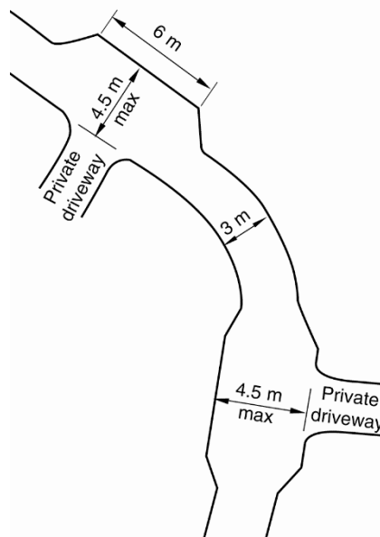
Figure 10.28 Passing areas
