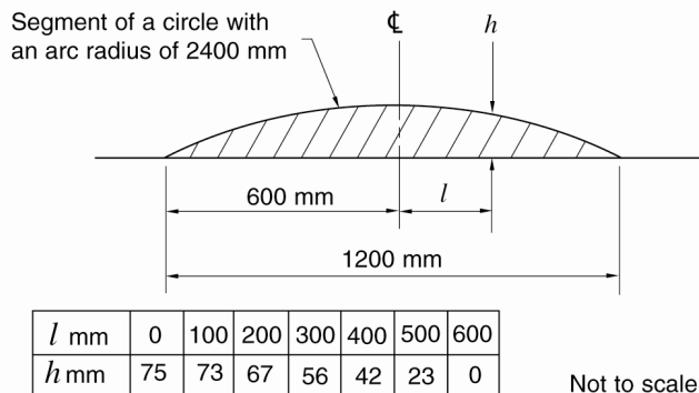
Figure 10.13 Off-street area Watt's profile road hump cross section
