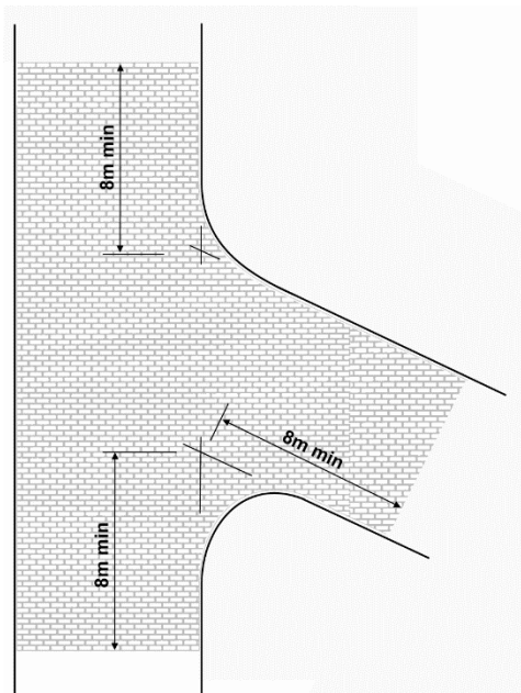
Figure 10.4 Contrasting pavement
