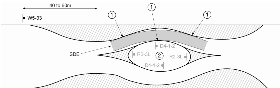
Figure 10.20 Centre blister on narrow roadway
