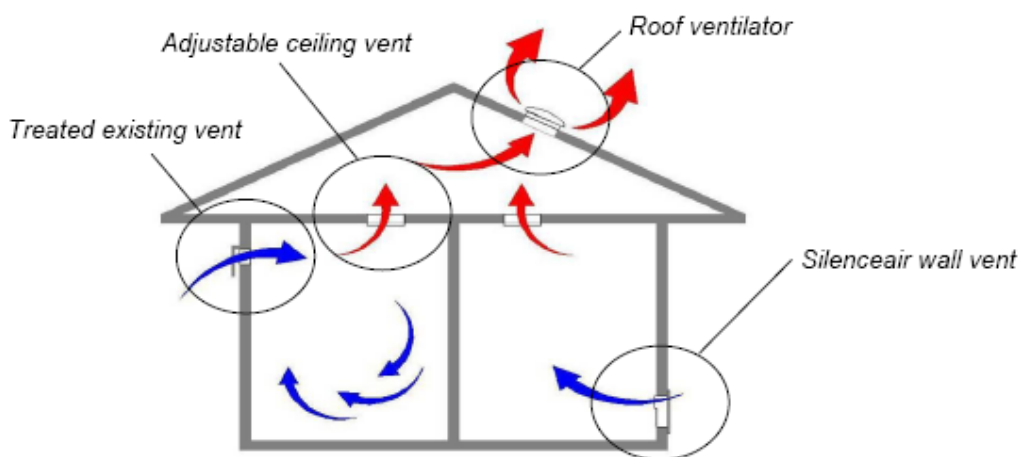
Roof space ventilators combined with ceiling vents remove air from the rooms, drawing fresh air in through wall vents
